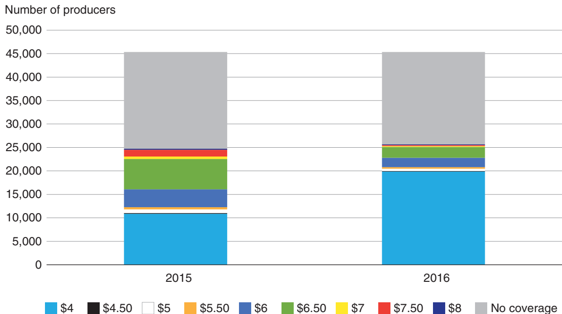
Figure 12 Enrollment by producers in the Dairy Margin Protection Program (MPP-Dairy) by coverage level ($/cwt) chosen, 2016
