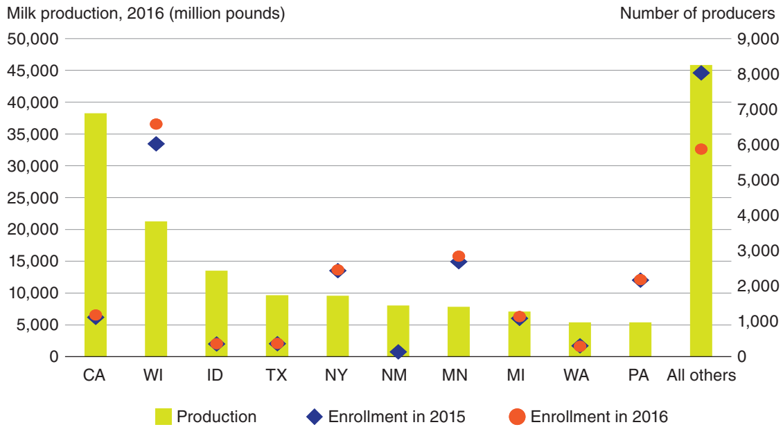
Figure 11 Milk production history and Dairy Margin Protection Program (MPP-Dairy) enrollment by State
