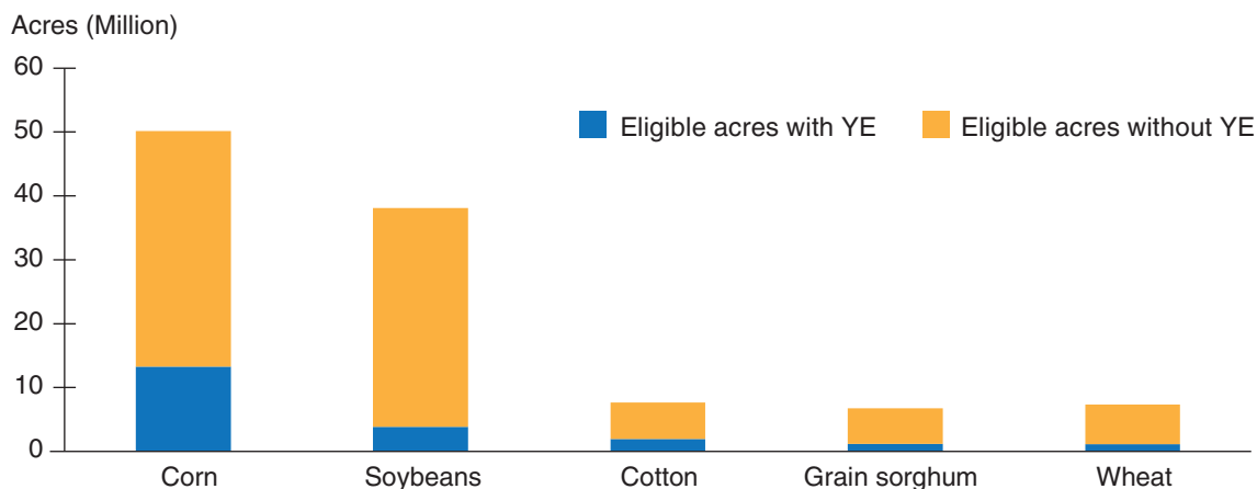
Figure 5 Insured acres eligible for yield exclusion (YE) by crop, 2015
